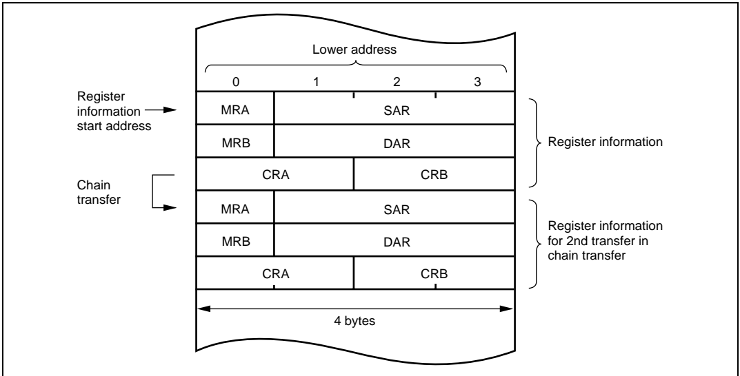
Figure 8.3 The Location of DTC Register Information in Address Space
