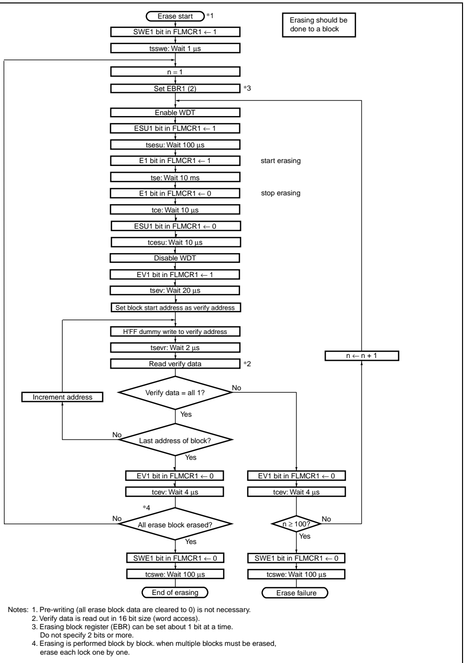
Figure 20.11 Erase/Erase-Verify Flowchart
